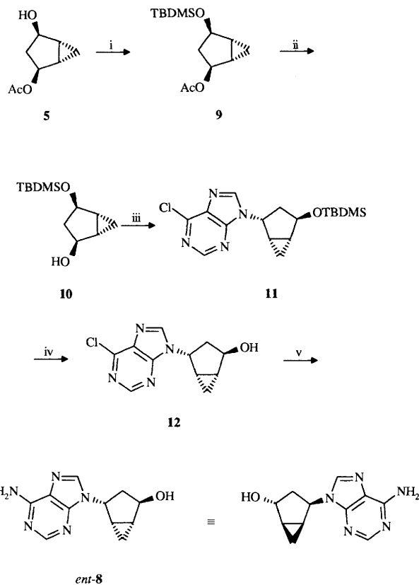
Scheme 3 Reagents and conditions: i, Bu t Me 2 SiCl, imidazole, DMF, room temp., 20 h, (99%); ii, ion-exchange resin Wofatit SBW (OH - ), MeOH, room temp., 35 h, (88%); iii, 6-chloropurine, DEAD, PPh 3 , THF, room temp., 2 h; iv, TBAF, THF, room temp., 2 h, (25% from 10 ); v, NH 3 , MeOH, 100 °C, 3 h (sealed bomb), (93%)
